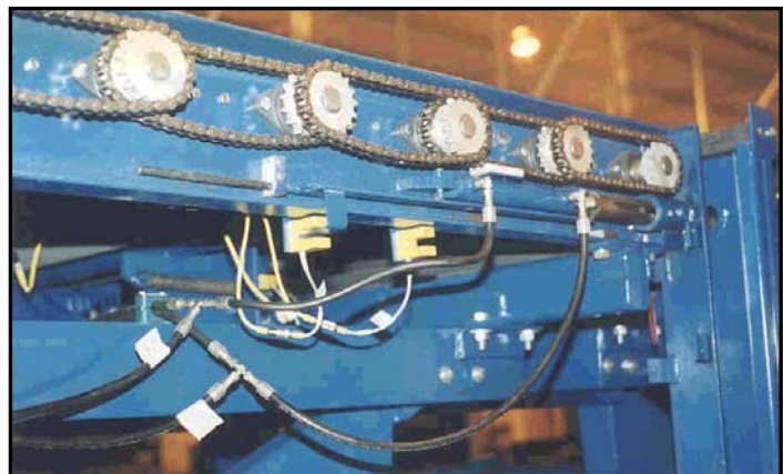
Typical Chain to Chain Roller Drive Set-up
